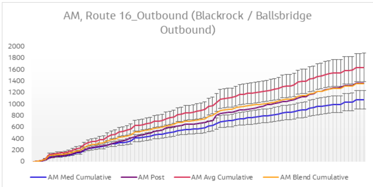
Diagram 6.13 Journey Time Validation Plot - Route 16 Outbound AM
