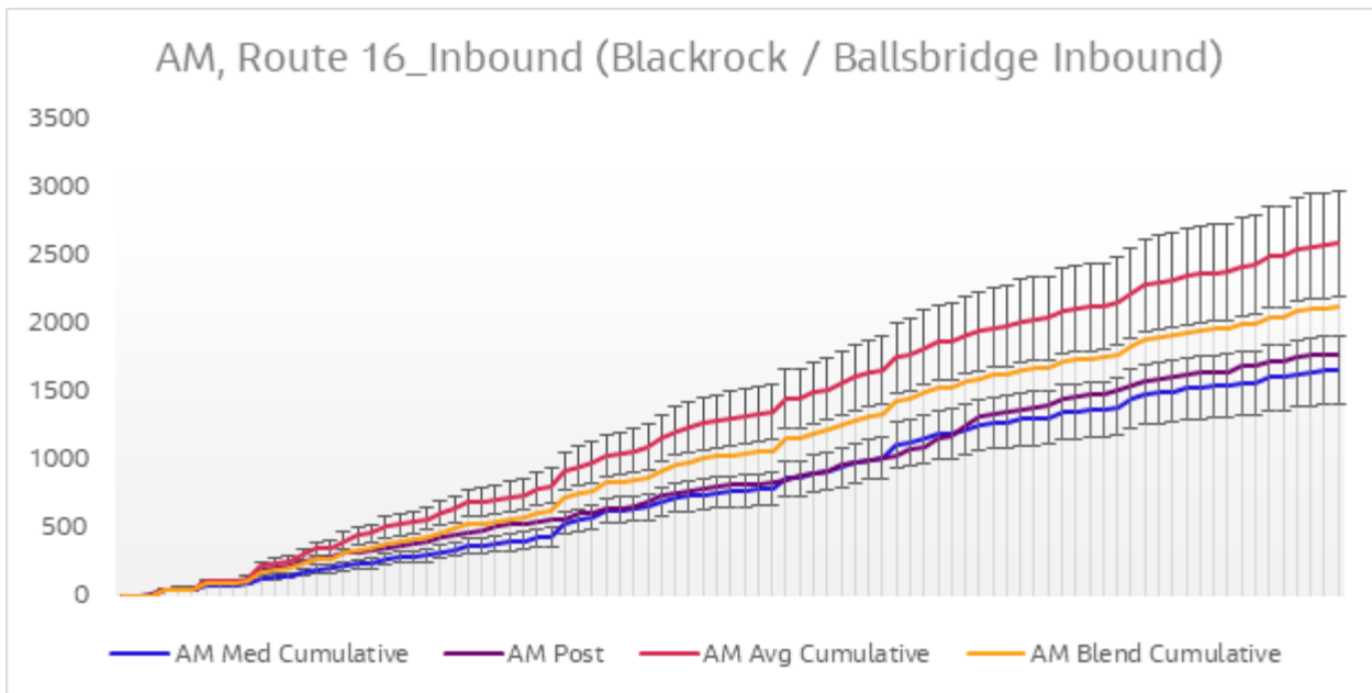
Diagram 6.12 Journey Time Validation Plot – Route 16 Inbound AM
