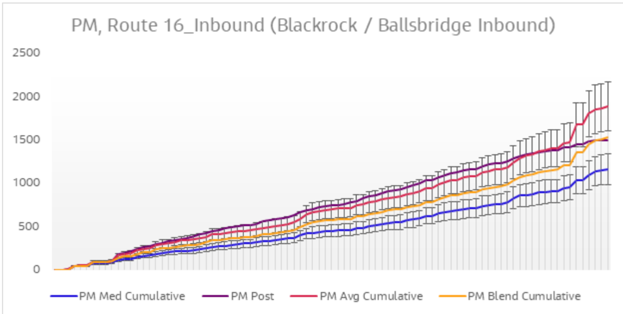
Diagram 6.18 Journey Time Validation Plot - Route 16 Inbound PM
