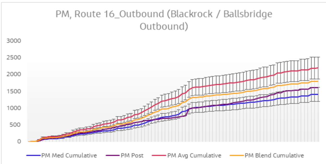
Diagram 6.19 Journey Time Validation Plot - Route 16 Outbound PM
