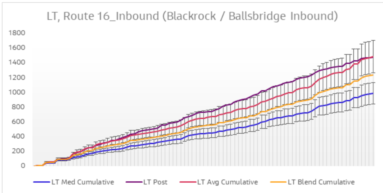
Diagram 6.14 Journey Time Validation Plot - Route 16 Inbound LT
