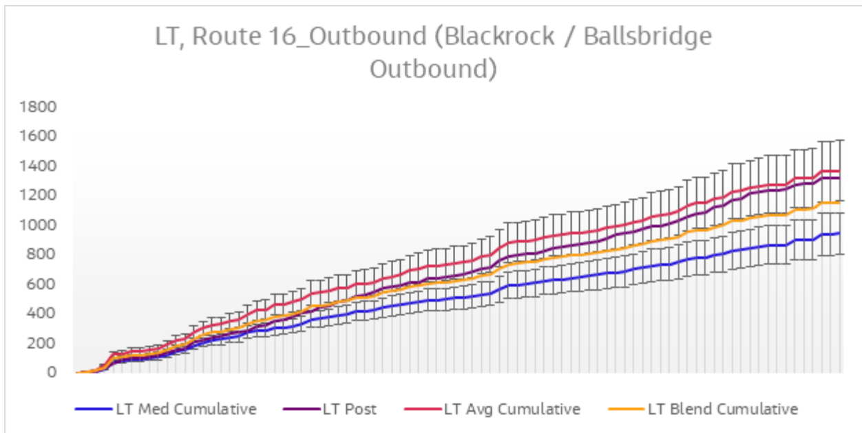
Diagram 6.15 Journey Time Validation Plot - Route 16 Outbound LT
