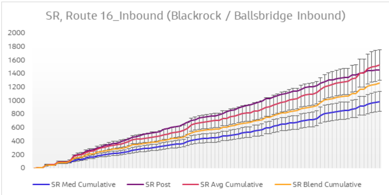
Diagram 6.16 Journey Time Validation Plot - Route 16 Inbound SR
