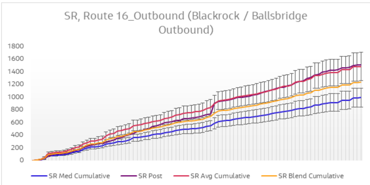
Diagram 6.17 Journey Time Validation Plot - Route 16 Outbound SR
